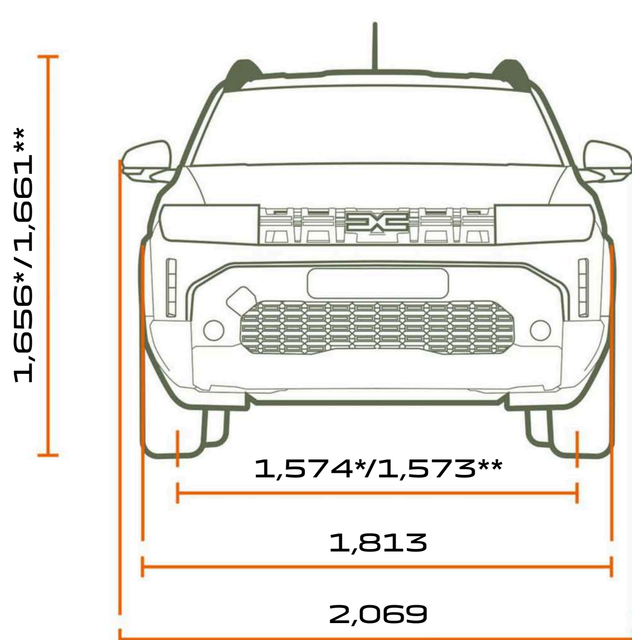
FRONT VIEW
