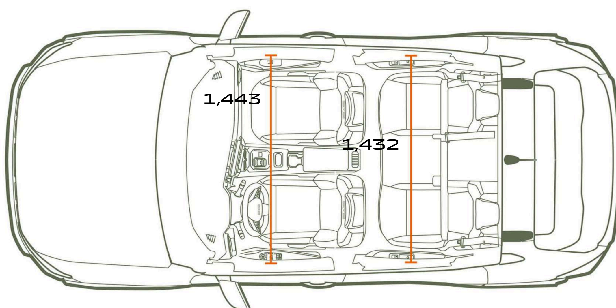
TOP VIEW
